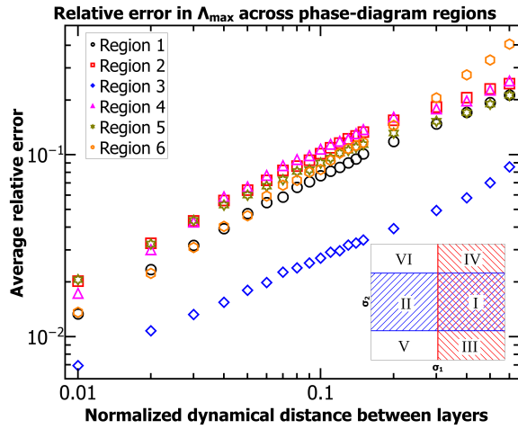
Figure 1. The accuracy of our theory increases with the ratio of the interaction strengths of the first layer \sigma_1 to that of the second layer \sigma_2 . The relative error in the estimate of the largest Lyapunov exponent \Lambda_{\max} of the perturbed system decreases from a maximum of approximately 40% in region 6 ( \sigma_1/\sigma_2 \approx 0.0917 ) to a minimum of approximately 0.7% in region 3 ( \sigma_1/\sigma_2 \approx 3.5 ). Within each region, the error increases sublinearly with the normalized dynamical distance. Each point is averaged over 1,000 realizations; error bars are smaller than the symbol size. Inset: schematic illustration of the six regions (adapted from del Genio et al. [27]). Layer 1 is individually stable only when \sigma_1 is greater than a critical value (red striped regions); layer 2 is individually stable only when \sigma_2 lies between two critical values (blue striped regions); region 1 is the only zone of the phase diagram where both layers are already individually stable.
