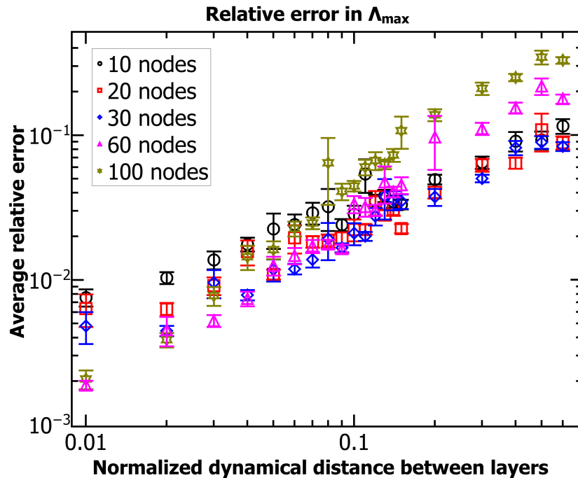
Supplementary Figure 3. The relative error in the largest Lyapunov exponent in preferential-attachment networks has no clear system-size dependence. The values of the average error in estimating the maximum Lyapunov exponent remain similar to those obtained for random networks, but without presenting a clear trend with network size. Also, the variability of the error is appreciably larger than it is for random networks. Each point is averaged over 1,000 realizations.
