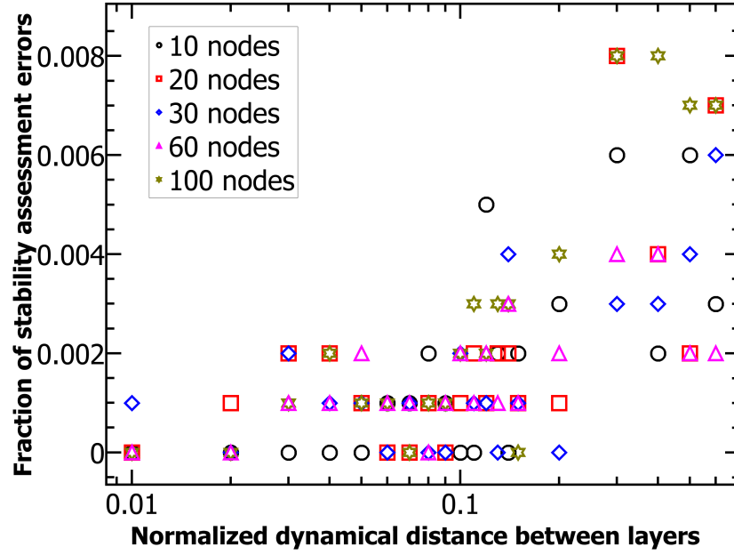
Supplementary Figure 2. Fraction of stability assessment errors in preferential-attachment networks. In networks with heterogeneous layer topology, the errors in assessing the synchronization stability no longer vanish. Nonetheless, their frequency remains very small, reaching a maximum of only 0.8% for normalized dynamical distances of at least 0.3. Each point is averaged over 1,000 realizations.
