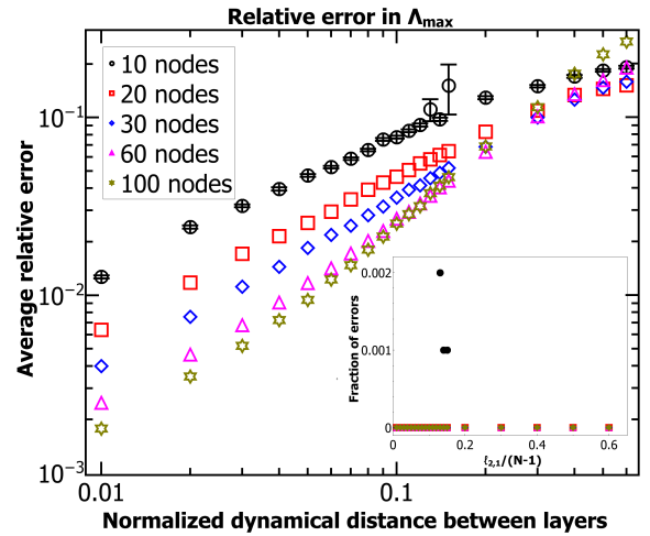
Figure 2. Synchronization stability of networks with multiple interaction layers is virtually always mean-field. In networks with N nodes per layer, for normalized dynamical distances \ell_{2,1}/(N-1) smaller than 0.1, the accuracy of the estimate of the maximum Lyapunov exponent \Lambda_{\max} improves with system size. Also, the error in the estimate never increases beyond 0.3, even for very large dynamical distances. Each point is averaged over 1,000 realizations; when not drawn, error bars are smaller than the symbol size. Inset: our mean-field theory assesses synchronization stability always correctly, with possible occasional exceptions only occurring in very small systems.
